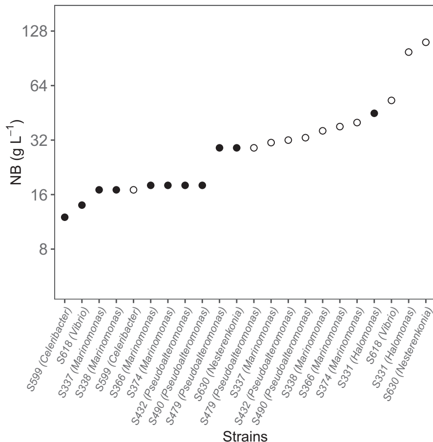
FIGURE 6 Ranking of the side-dependent niche breadths (NB) for the 11 model strains. Black dots indicate hyperosmotic NB, while white dots indicate hypoosmotic NB. The y-axis is displayed on a log-scale
