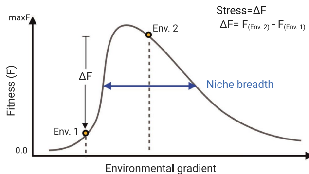
FIGURE 1 Schematic illustration for NB estimation and stress exposure. The NB is a constant parameter for each species defined as the length of the environmental gradient covered by the fitness curve of the species at a given fitness value. Stress is quantified as the difference in fitness between any pair of environments E1 and E2. Depending on the position of Env.1 and Env.2 along the environmental gradient, stress can take all values between 0 and the maximum fitness value maxF. We hypothesized that the NB and accordingly the stress an organism is exposed to after environmental change is linked to general patterns of its transcriptional response, which eventually is manifested in the organism's physiological response to changing environmental conditions
